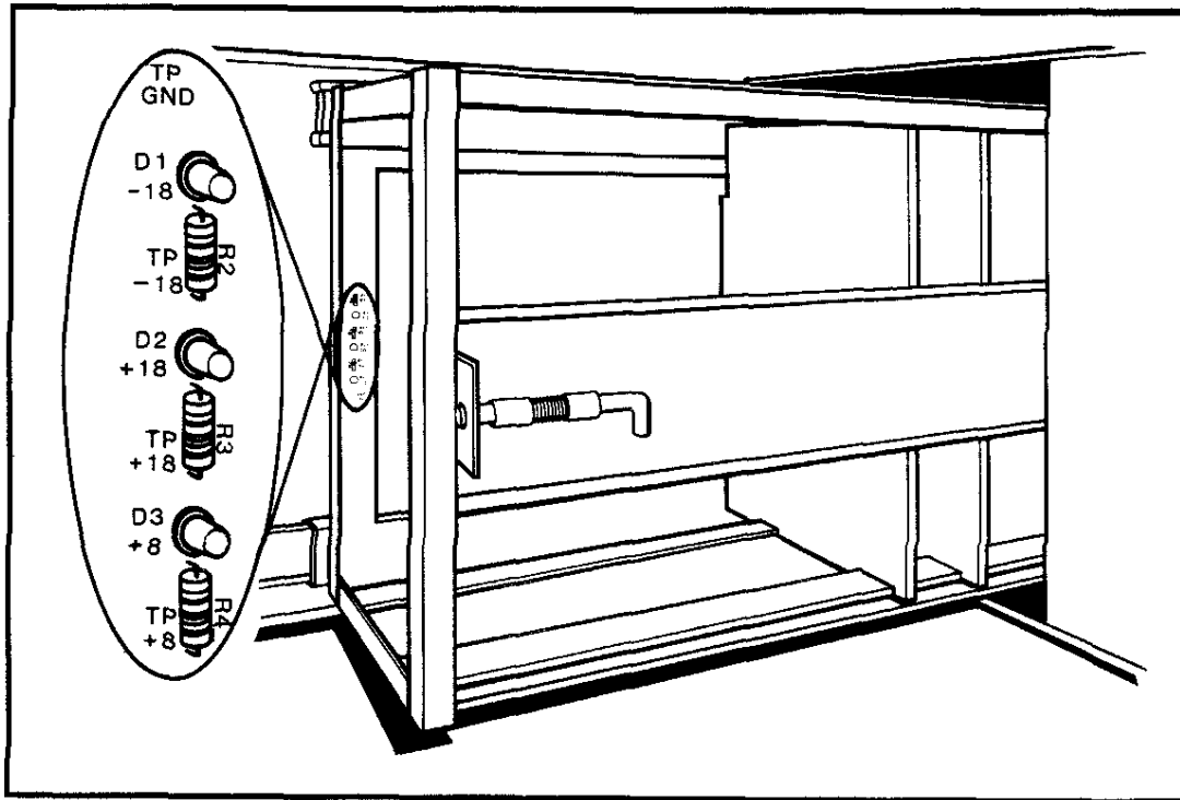
Figure D-3: LOCATION OF POWER SUPPLY LEADS
