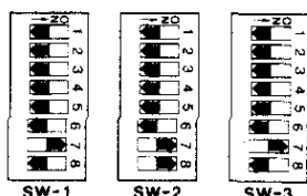
Figure F-3: SWITCH SETTINGS FOR 64KZ-II BOARDS IN CROMIX OPERATING SYSTEMS
